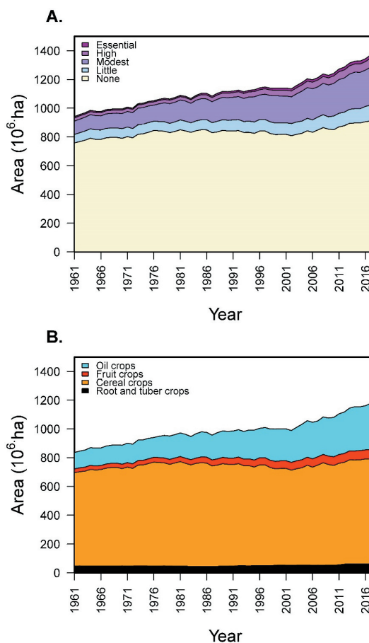
Figure 4. Global temporal trends (1961–2018) in agricultural area planted with (A) crops with different dependence on pollinators (none [0%], little [ >0 and <10\% ], modest [ >10 and <40\% ], high [ >40 and <90\% ], essential [ >90\% ]) (Klein et al. 2007), and (B) oil, fruit, cereal, and root and tuber crops (FAOSTAT 2021).
