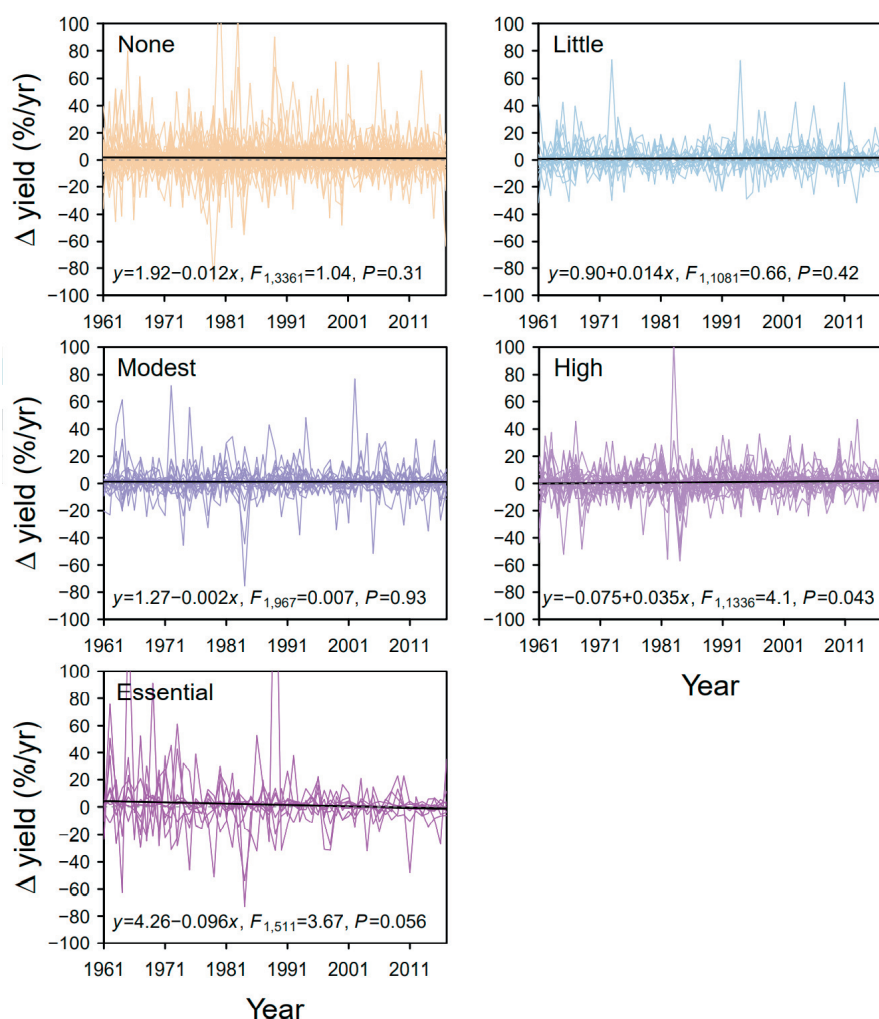
Figure 3. Global temporal trends in annual growth rates in yield between 1961 and 2018 for 128 crops with complete yield records (FAOSTAT 2021) categorized by pollinator dependence based on the percentage of yield reduction in the absence of pollinators (none [0%, n=59 crops], little [ >0 and <10\% , n=19], modest [ >10 and <40\% , n=17], high [ >40 and <90\% , n=24], essential [ >90\% , n=9]). Annual growth rates in yield were estimated using the equation in Figure 1. Rates calculated from change between consecutive years simplifies to percent change, 100 * [(x_{t+1}/x_t) - 1] , where x_t and x_{t+1} are yield values in t/ha during years t and t+1, respectively. The solid black line depicts the regression of annual yield growth rate vs. year (1961=year 0) for each pollinator-dependent category and the grey dashed line at 0 indicates yield constancy. The interaction between year and pollinator dependence (i.e., using the mid value for each dependence category (none [0%], little [5%], modest [25%], high [65%], essential [95%]) in a regression model that considered both predictors did not detect a temporal relation with increasing pollinator dependence ( F_{1,7292} = 0.23 , P = 0.64 ). Including 'crop' as a random effect did not improve the fit of any model. Models were implemented with the statistical software R version 4.0.2 (R Core Team 2020) using the lm function of the basic library and the lmer function of the lme4 library (version 1.1-23) (Bates et al. 2015).
