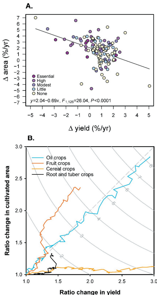
Figure 5. Relations of annual growth in global cultivated area to growth in global yield between 1961 and 2018 based on data from FAOSTAT (2021). In (A) the solid line depicts the regression of mean annual growth in cultivated area to mean annual yield growth for 128 crops categorized by pollinator dependence (none [0%, n=59 crops], little [ >0 and <10\% , n=19], modest [ >10 and <40\% , n=17], high [ >40 and <90\% , n=24], essential [ >90\% , n=9]). Adding pollinator-dependence as a categorical factor did not provide evidence that the depicted negative relation varies among pollinator dependence categories (yield growth x pollinator dependence interaction, F_{4,118} = 0.29 , P = 0.88 ). The models were implemented using the lm function of the basic library statistical software R version 4.0.2 (R Core Team 2020). In (B) the growth trajectories depict the ratio change in cultivated area and yield for oil, fruit, cereal, and root and tuber crops based on 1961 values. The dashed gray diagonal line represents proportional change in area and yield ratios. The gray curves depict isoclines for the ratio change in total production (area x yield) as indicated by the associated number.
