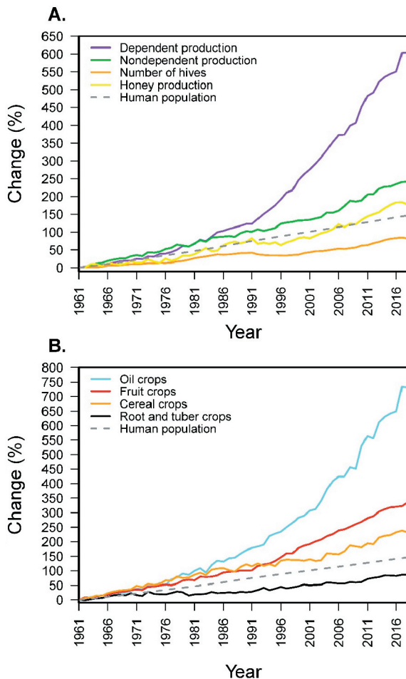
Figure 2. Global temporal trends (1961-2018) in (A) the fractions of agricultural production that depend and does not depend on pollinators (estimated following the methodology of Aizen and Harder 2009a), the number of honey-bee hives, and honey production, and (B) total production by oil, fruit, cereal and root and tuber crops (FAOSTAT 2021). The trend in the size of the human population is included in both panels as a reference. Change for each variable x from 1961 until year t is calculated as a percentage of the 1961 value. Absolute values during 1961 were: agricultural production that depended on pollinators= 117.19 \times 10^6 t; agricultural production that did not depend on pollinators= 2324.41 \times 10^6 t; number of honey-bee hives= 49.17 \times 10^6 hives; honey production= 0.678 \times 10^6 t; oil crops= 132.15 \times 10^6 t; fruit crops= 199.84 \times 10^6 t; cereal crops= 876.87 \times 10^6 t; root and tuber crops= 455.31 \times 10^6 t, and human population= 3901.84 \times 10^6 individuals.
