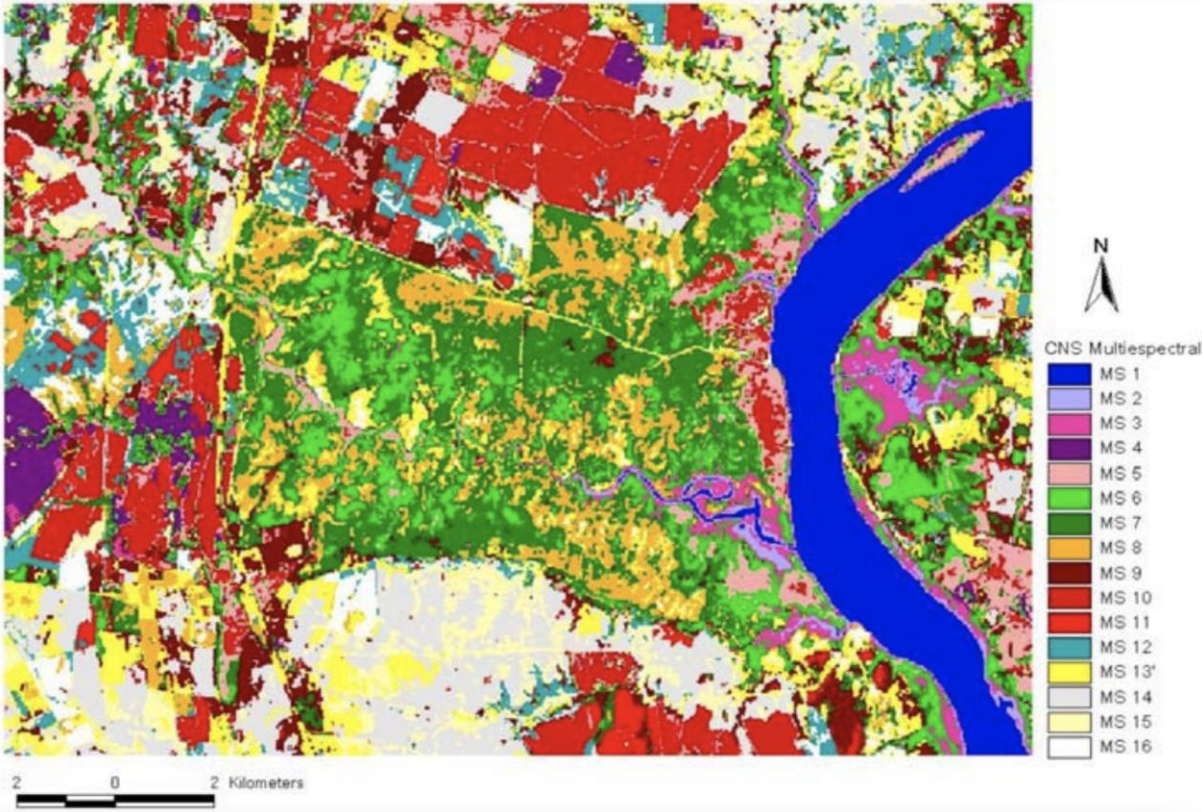
Figure S2. Unsupervised classification of the multispectral multitemporal image (Ruiz Selmo et al. 2007).
